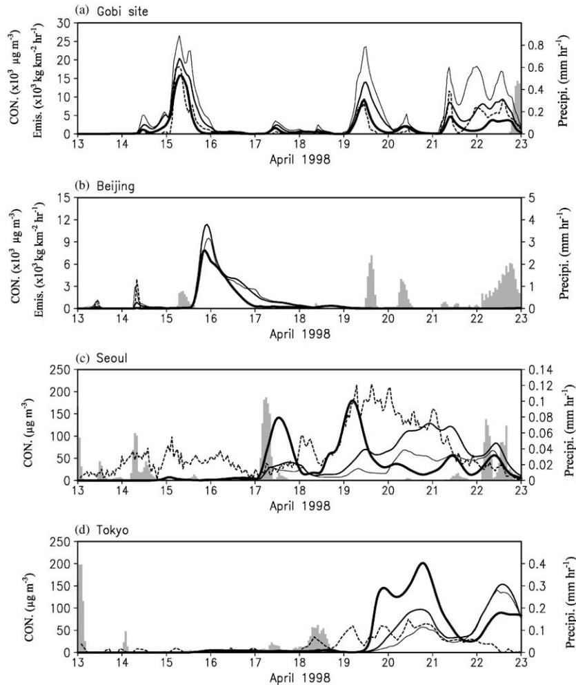
Fig. 8. The time series of modeled mean dust concentration ( \mu\text{g m}^{-3} ) averaged for the layers of surface to 100 m (—), 100–1000 m (---), and 1000–3000 m (—) with precipitation rate ( \text{mm h}^{-1} ) at (a) Gobi site, (b) Beijing, (c) Seoul, and (d) Tokyo. Emission rates ( 10^3 \text{ kg km}^{-2} \text{ h}^{-1} ) at the Gobi site and Beijing and the observed TSP concentrations (----) at Seoul and Tokyo are also shown.
